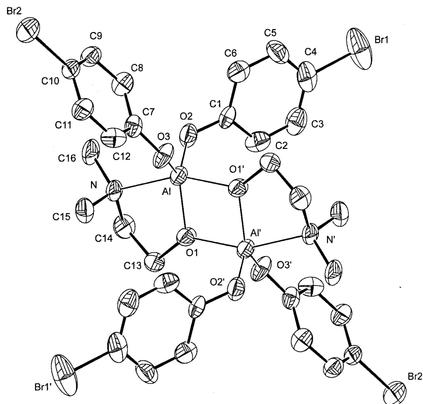
Figure 1. ORTEP diagram of 7 ; thermal ellipsoids are shown at the 30% probability level; hydrogen atoms are omitted for clarity; selected bond lengths (Å) and bond angles (°): Al–O(1) 1.813(8), Al–O(1') 1.879(8), Al–O(2) 1.727(9), Al–O(3) 1.726(8), Al–N 2.097(9); Al–O(1)–Al' 104.5(4), O(1)–Al–N 81.5(4), O(1)–Al–O(2) 120.2(4), O(1)–Al–O(3) 121.8(4), O(1')–Al–N 157.0(4), O(1')–Al–O(2) 100.6(4), O(1')–Al–O(3) 93.0(4), O(2)–Al–O(3) 118.0(4), N–Al–O(2) 91.5(4), N–Al–O(3) 98.6(4); symmetry transformation used to generate equivalent atoms: (') -x + 1, -y + 1, -z + 1
